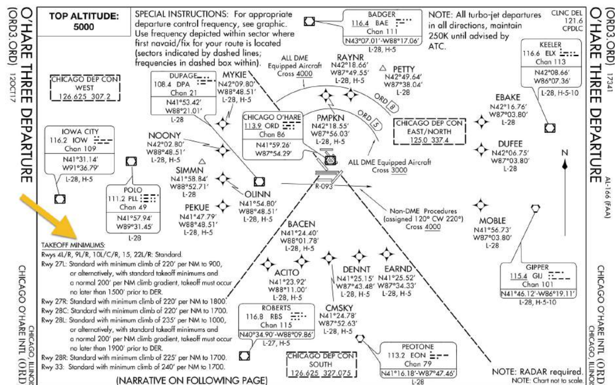
Figure 5.21. Civil SID.
