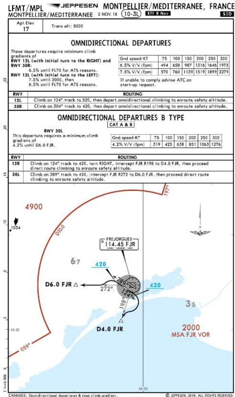
Figure 5.6. Omnidirectional Departure.
