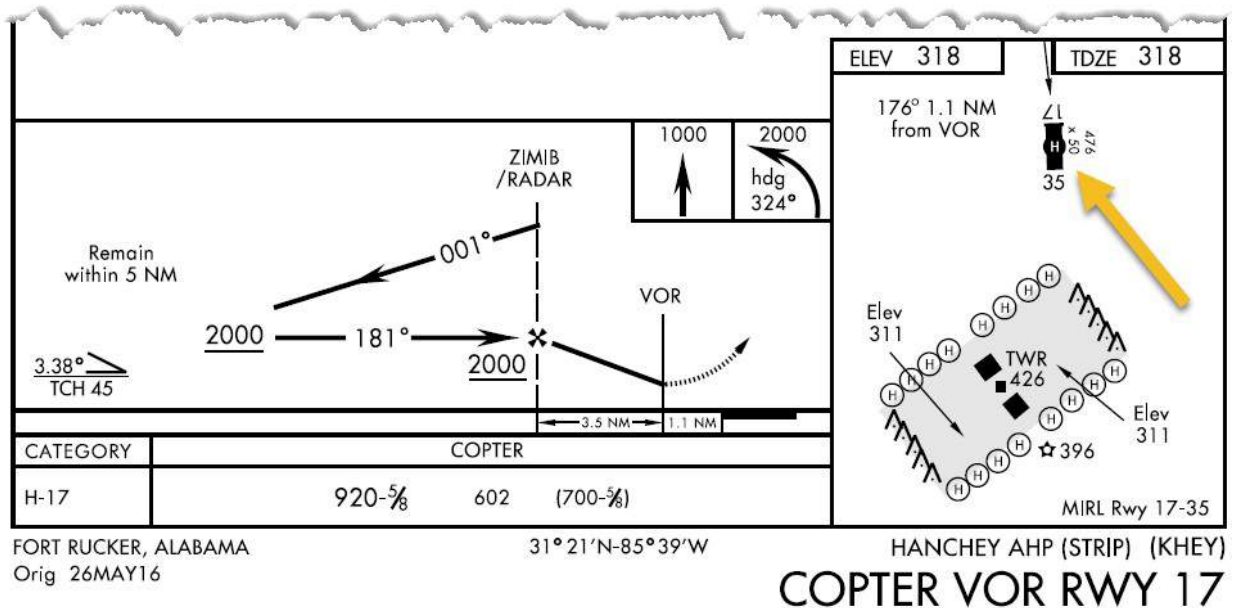
Figure 15.30. Helicopter-Only Approach.
