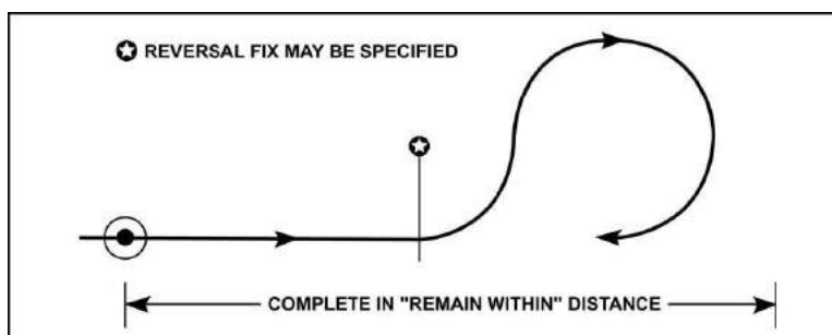
Figure 15.22. 80°/260° Procedure Turn.
